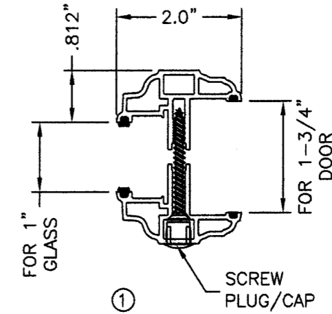
ODL/WESTERN REFLECTION HURRICANE LIGHT FRAME KIT EXTRUDED ALUMINUM 0.070" MIN. WALL THK. ALUMINUM ALLOY - 6063-T5
