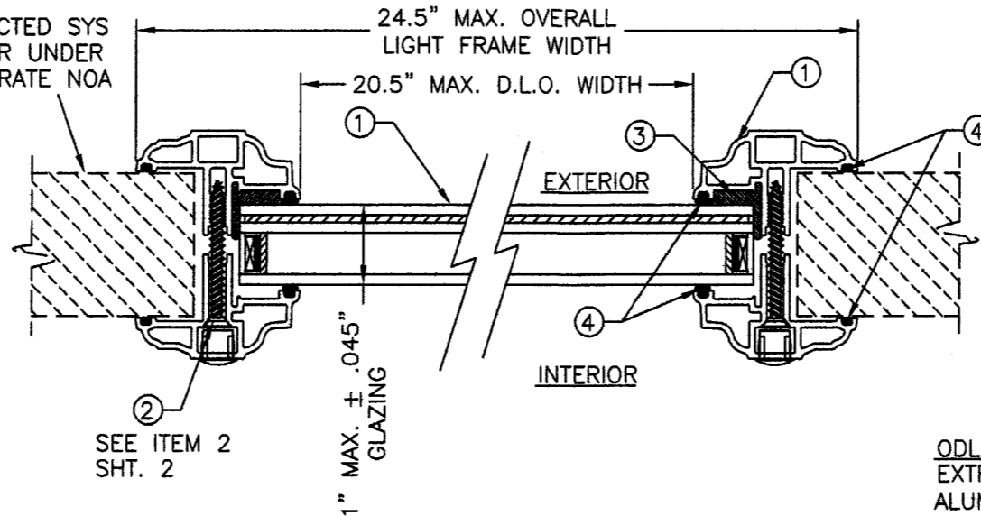
2 HORIZONTAL CROSS SECTION
