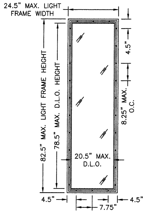
ODL/WESTERN REF. ALUMINUM LIGHT KIT ASSEMBLY 8'0" UNITS
