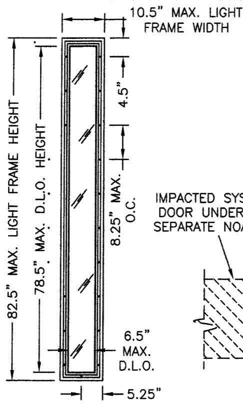
ODL/WESTERN REF. ALUMINUM LIGHT KIT ASSEMBLY 8'0" UNITS
