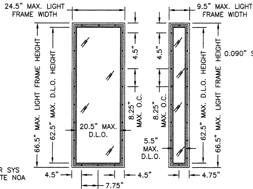
ODL/WESTERN REF. ALUMINUM LIGHT KIT ASSEMBLY 6'8" UNITS
