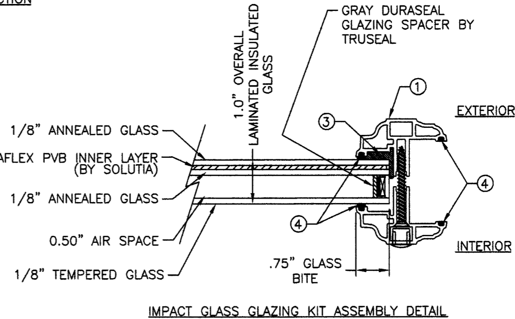
ODL/WESTERN REFLECTION HURRICANE LIGHT FRAME KIT EXTRUDED ALUMINUM 0.070" MIN. WALL THK. ALUMINUM ALLOY - 6063-T5
