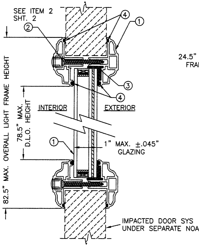
1 VERTICAL CROSS SECTION
